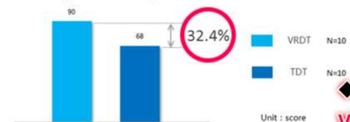
◆図3 Average Score of Delay Test
